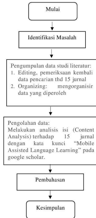
Gambar 1. Alur Penelitian
