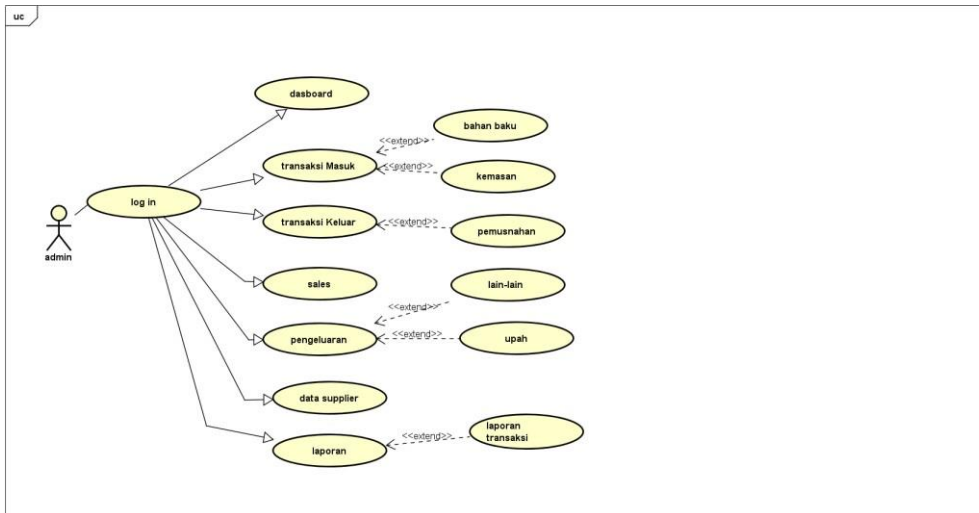
Gambar 4.1 usecase diagram
