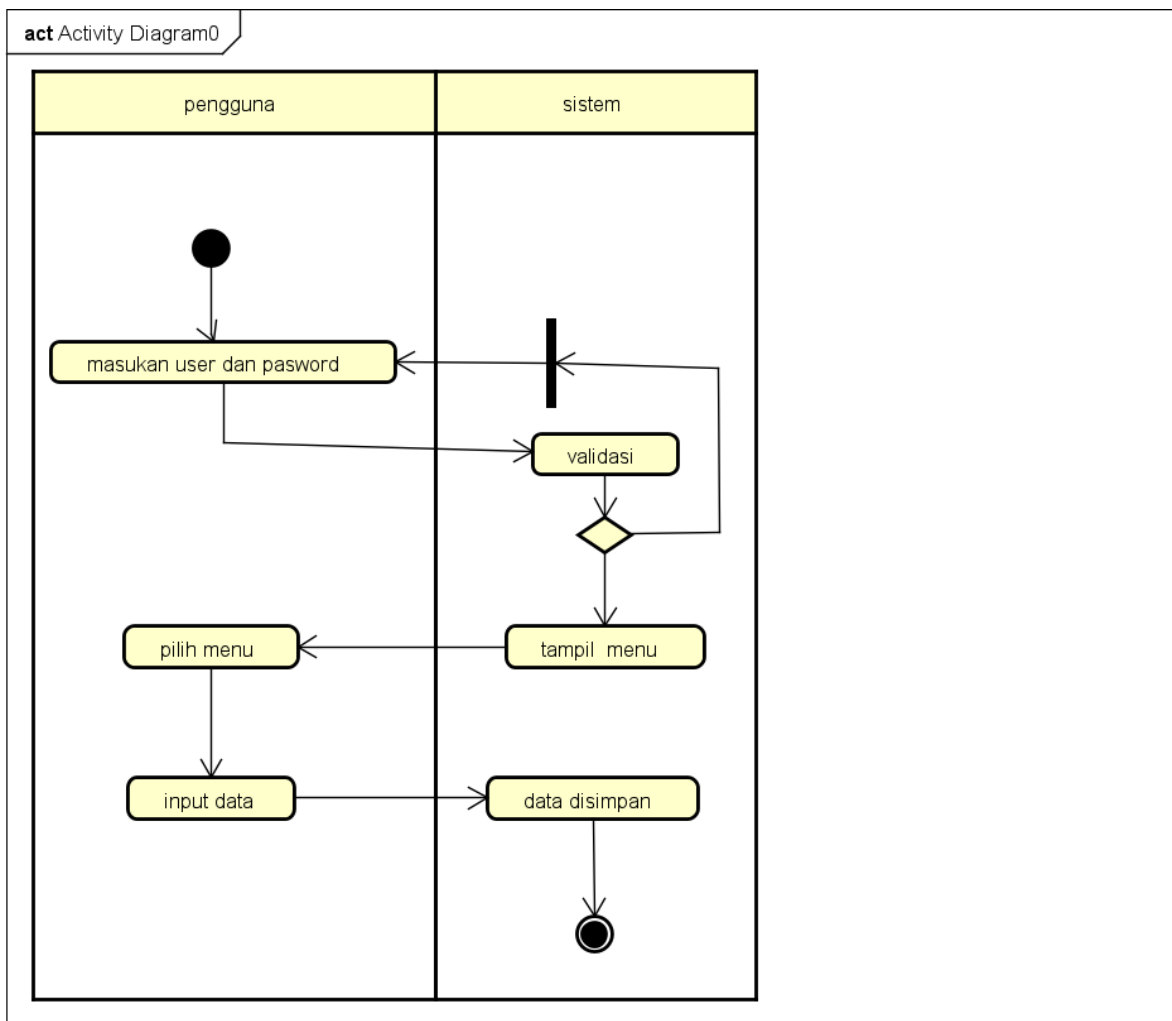
Gambar 4.2 Usecase activity
